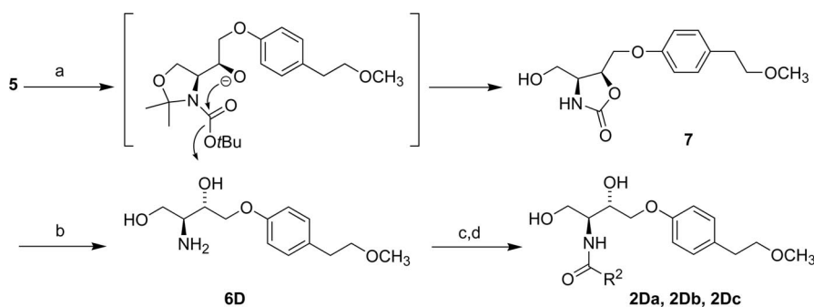
Scheme 2. Reagents and conditions: (a) NaH, p -[CH 3 O(CH 2 ) 2 Ph-OH ( D ), DMF, followed by steps b–e (Scheme 1); (b) 2 N NaOH/EtOH, 80 °C; (c) PS-EDC, R 2 COOH ( a–c ), CHCl 3 / t BuOH, r.t.; (d) Amberlyst A21, DCM, r.t.
